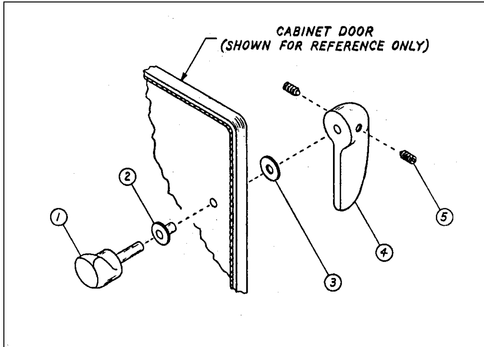
Figure 1. Cabinet Door Handle—Exploded View
